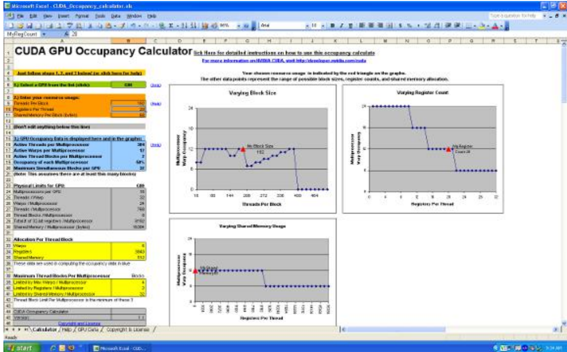
Figure 11 Using the CUDA Occupancy Calculator to project GPU multiprocessor occupancy
